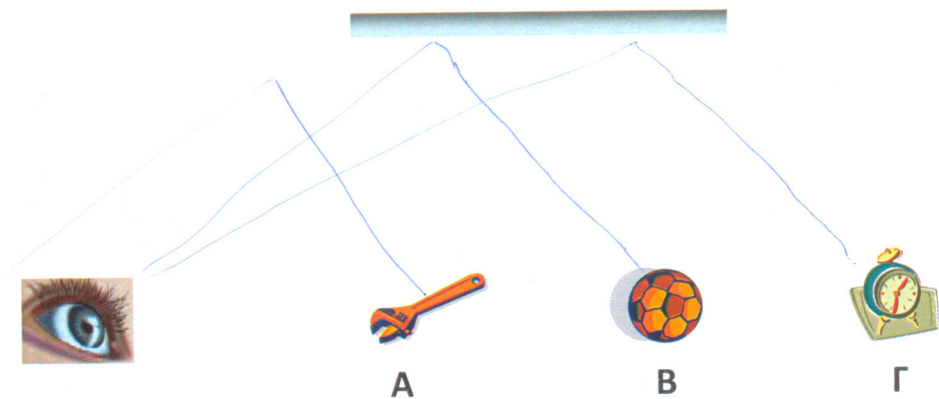
Figure 4. Correct scientific application of the ray model.
