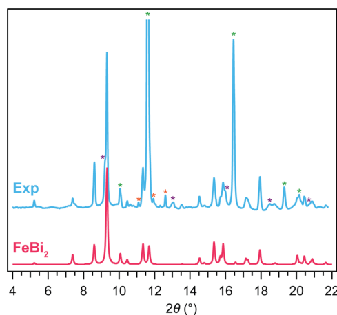
Figure 2. Background-subtracted X-ray diffraction pattern of the reaction site after cooling to room temperature ( \lambda = 0.406626\ \text{\AA} , P = 29.9(1) GPa). The experimental trace is plotted in blue, with asterisks denoting the peaks arising from MgO (green), unreacted Bi(V) (purple), and unreacted \epsilon -Fe (orange). The simulated pattern of \text{FeBi}_2 based on the final fit parameters is plotted in pink.
