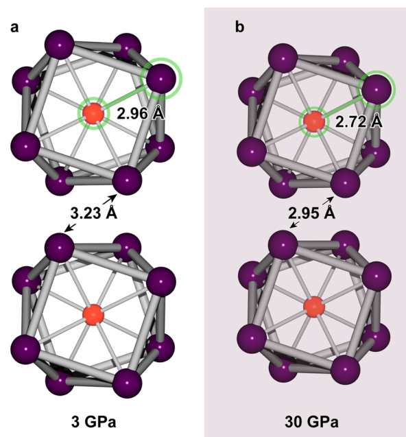
Figure 3. View down the c -axis at 3 GPa (a) and 30 GPa (b), illustrating the effect of increased pressure on the Fe–Bi interaction and the intercolumn Bi–Bi interaction. Purple and orange spheres represent Bi and Fe atoms, respectively.
