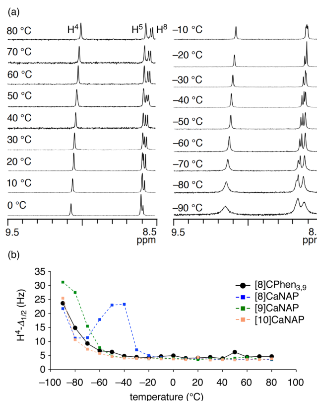
Figure 7. VT NMR analysis of [8]CPhen 3,9 . (a) Spectra of the aromatic region showing representative 1 H resonances in toluene- d 8 . See Figure S3 for the whole aromatic region. (b) Temperature dependence of full width at half-maximum ( \Delta_{1/2} ) of the H 4 resonance. Reference data of [ n ]CaNAP ( n = 8–10) were taken from ref 20.
