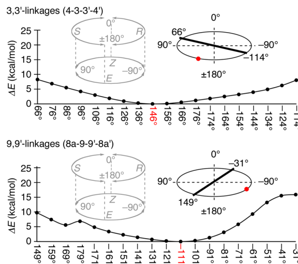
Figure 5. Energy profiles of the biaryl rotation in [8]CPhen 3,9 from scan calculations at the semiempirical PM6 level of theory. The dihedral angle was scanned for 180^\circ rotations in \pm 10^\circ increments.
